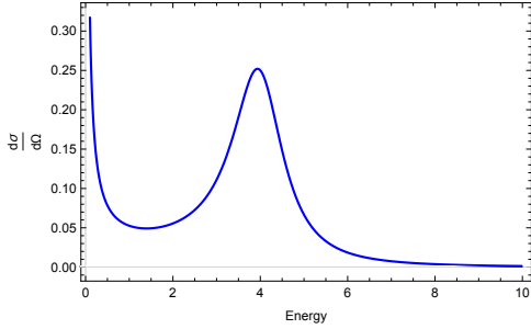
Figure 100: Distribution with \Gamma^2 = 2\dots
